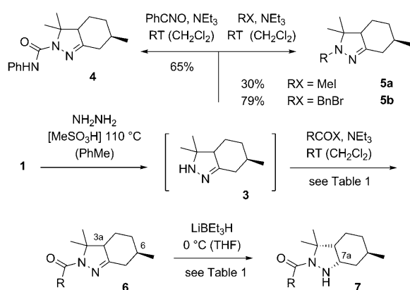
Scheme 2. Access to various N(2)-substituted hexahydroindazoles 4–6 from the known intermediate 3 and reduction of the N(2)-acyl derivatives 6 to octahydroindazoles 7 .
