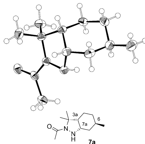
Figure 2. A molecule of compound 7a in the crystal.
