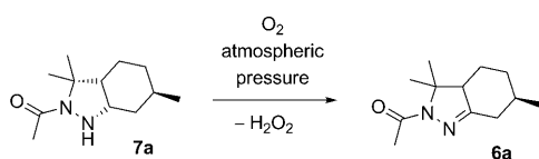
Scheme 7. Oxidation of octahydroindazole 7a to hexahydroindazole 6a with concomitant formation of hydrogen peroxide.
