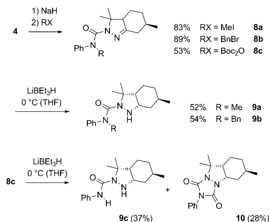
Scheme 3. N-Alkylation and N-acylation of the secondary carbamate 4 to hexahydroindazoles 8 , which were further reduced with lithium triethylborohydride.
