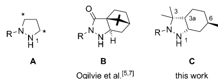
Figure 1. General structure of a chiral pyrazolidine A , of the chiral pyrazolidinones B earlier described by Ogilvie et al. [5,7] and of the N(2)-substituted pyrazolidines C (octahydroindazoles), which are discussed in this report.
