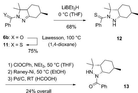
Scheme 4. Synthesis of the N(1)-benzoylated octahydroindazole 13 from N(2)-benzoylated hexahydroindazole 6b via thioamide 12 .
