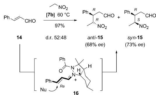
Scheme 6. Enantioselective preparation of Michael addition products anti - 15 and syn - 15 and presumed structure of the iminium ion intermediate 16 formed from aldehyde 14 and octahydroindazole 7b .
