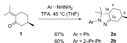
Scheme 1. Acid-promoted condensation of (+)-pulegone ( 1 ) and aromatic hydrazines to hexahydroindazoles 2 .
