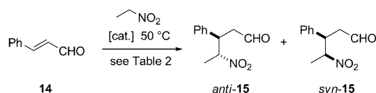
Scheme 5. Michael addition of nitroethane to cinnamaldehyde ( 14 ) leading to the two diastereomeric addition products anti - 15 and syn - 15 .
