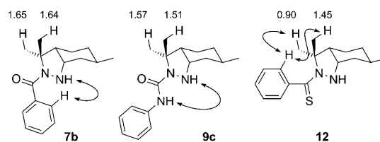
Figure 3. 1 H NMR chemical shift data of the gem -dimethyl substituents at C(3) and significant 1 H-NOESY contacts in octahydroindazoles 7b , 9c , and 12 .
